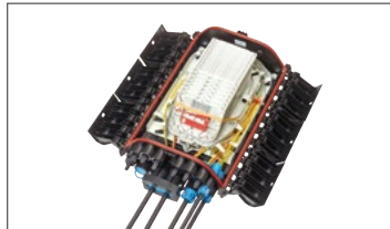
BPEO Closure Size 2
