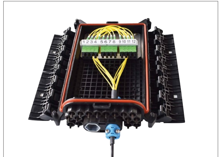
MiniXtend Cable with Binderless FastAccess Technology
