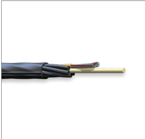
24-Fibre MiniXtend Cable with Binderless FastAccess Technology
