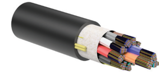
Corning® RocketRibbon® Cable
